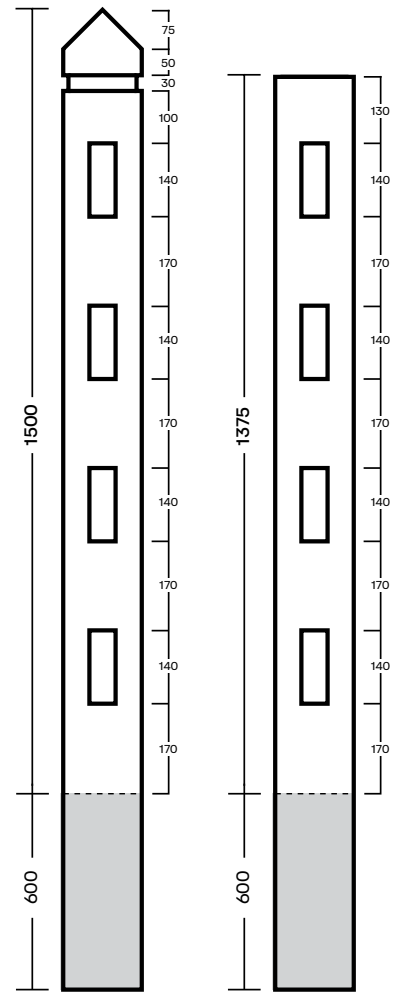
Four Rail
