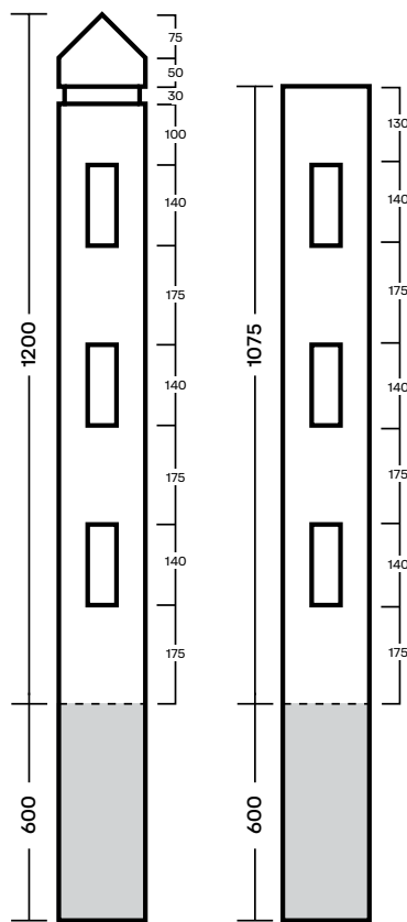
Three Rail
